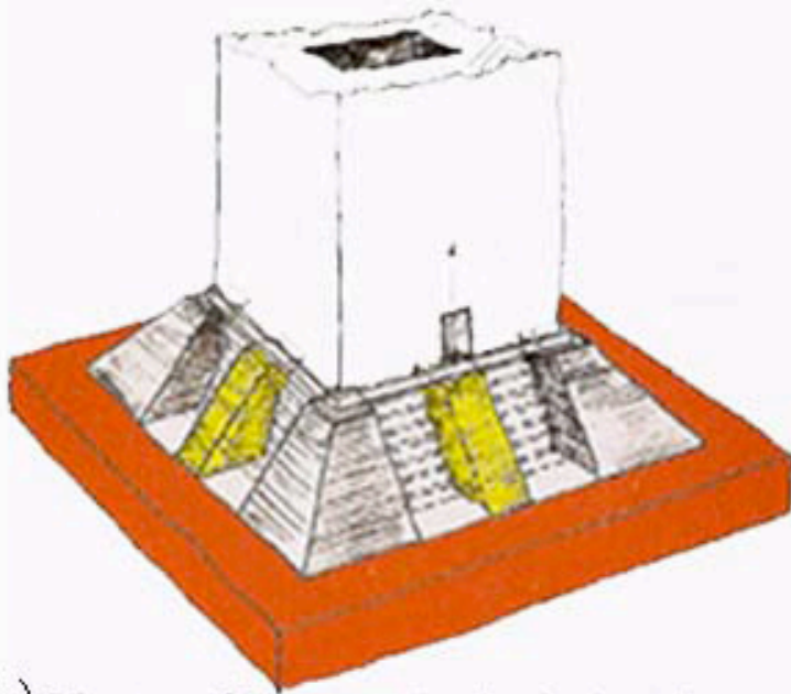
(a) Diagram of Monument underpinning plan.
