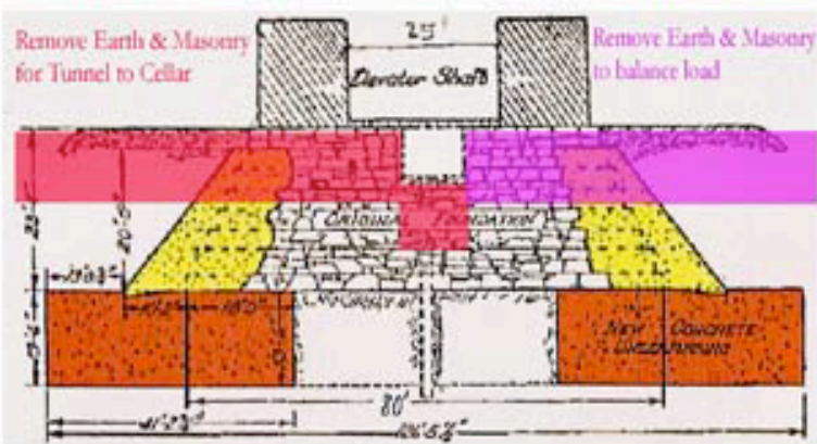
(c) Diagrammatic Section Showing Excavation Through Buttresses and Foundation
